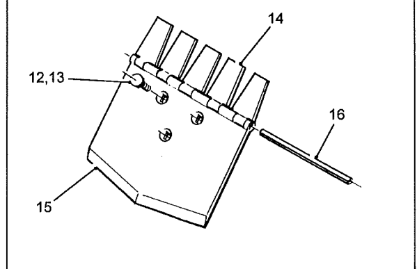
Centre Share Assembly - Assy No 51295
