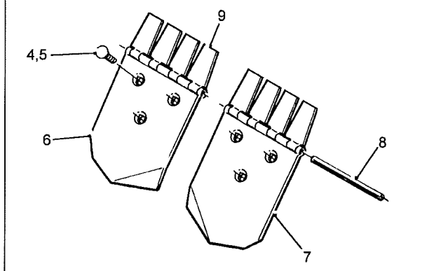
2 Row Share Assembly - Assy No 51294
