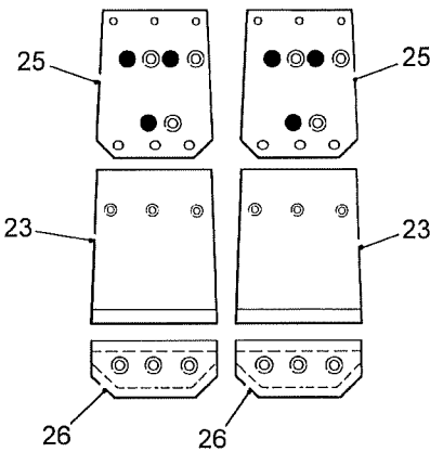
Plastic Shares For 32" Rows
