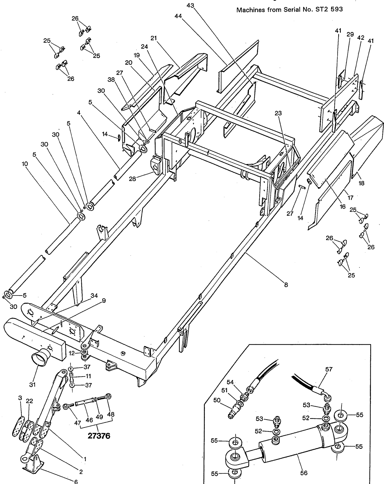
Hydraulic Ram Assembly - 27377
