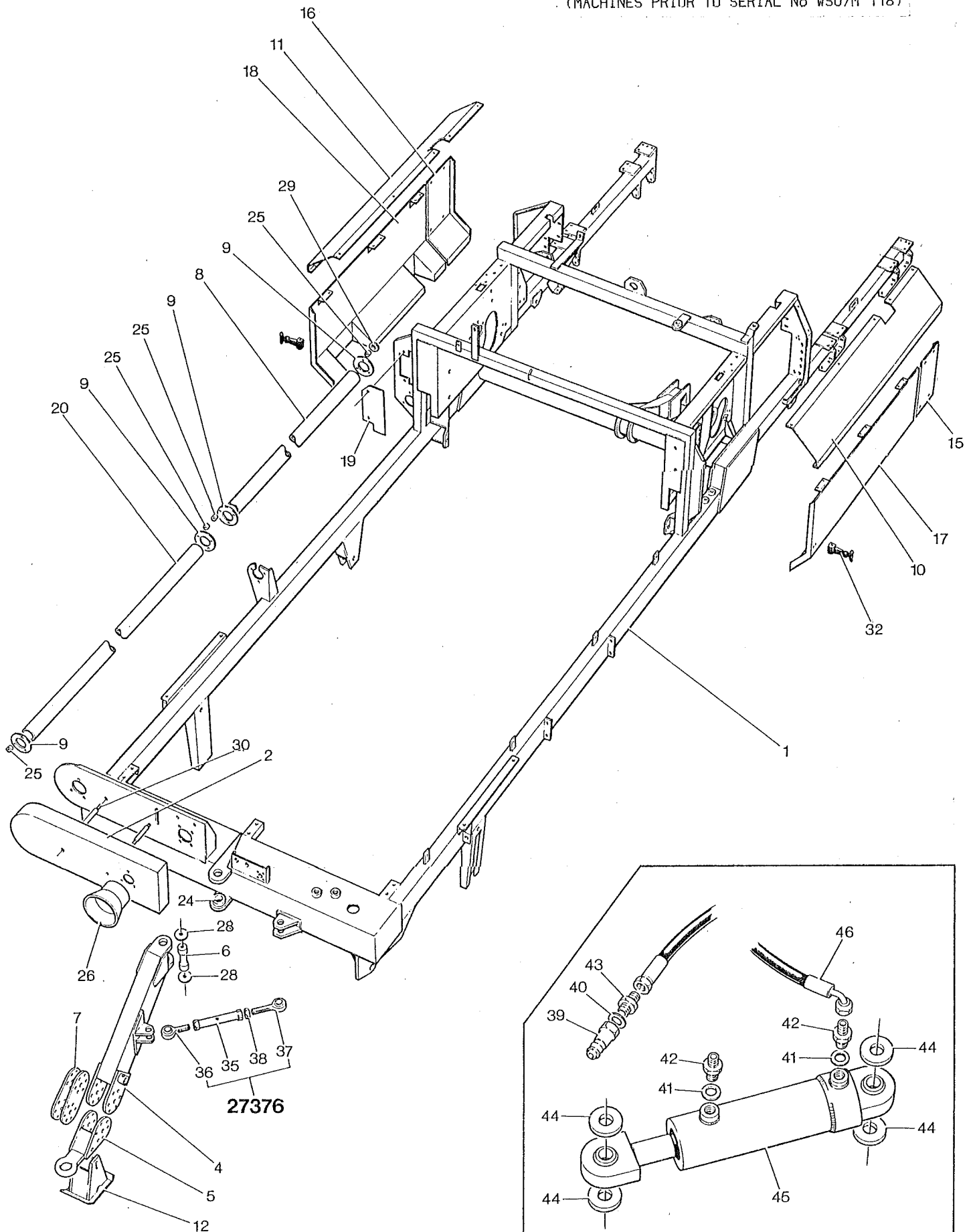
Hydraulic Ram Assembly - 27377
