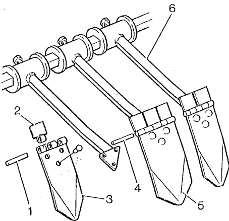
Three Piece Share Assembly for Wide Diablo Rollers — Assy N° WO693
