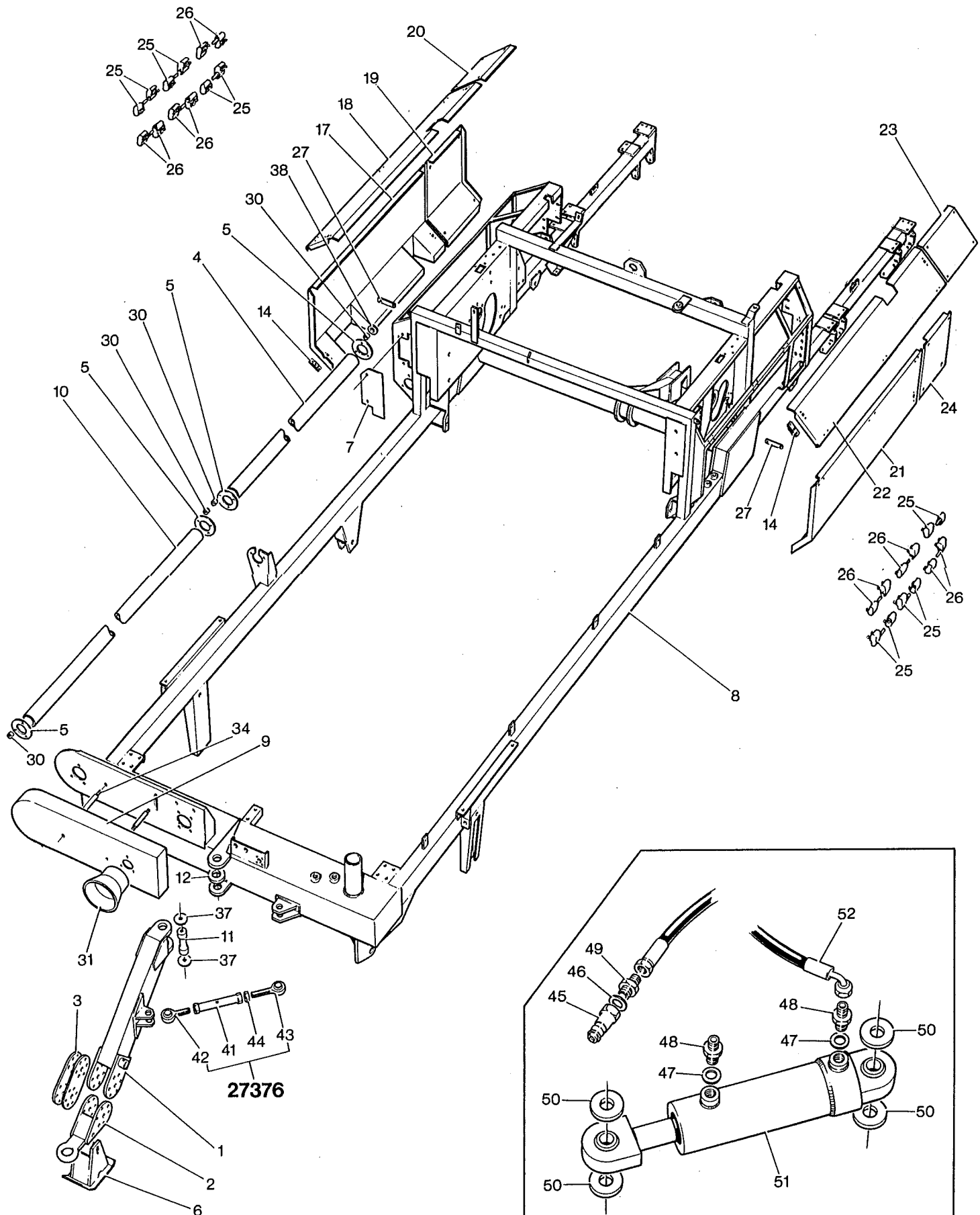
Hydraulic Ram Assembly - 27377
