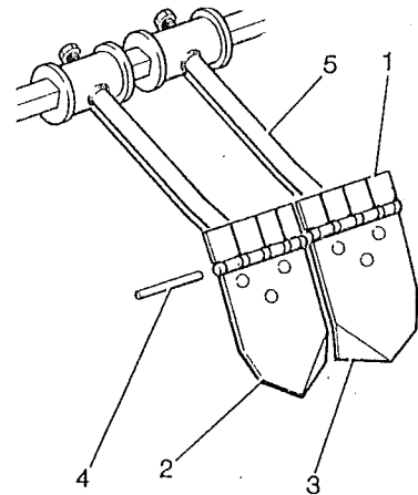
Two Piece Share Assembly— Assy N° 27883
