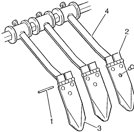
Three Piece Share Assembly for Narrow Diablo Rollers — Assy N° WO691
