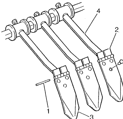
Three Piece Share Assembly for Bed Work with Half Diablo Rollers — Assy N° 27973
