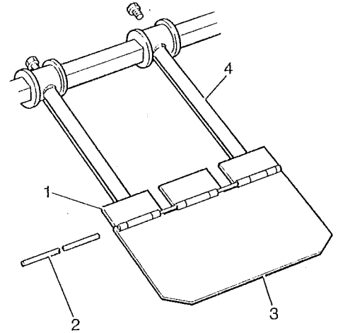
Single Piece Share Assembly— Assy N° WO692
