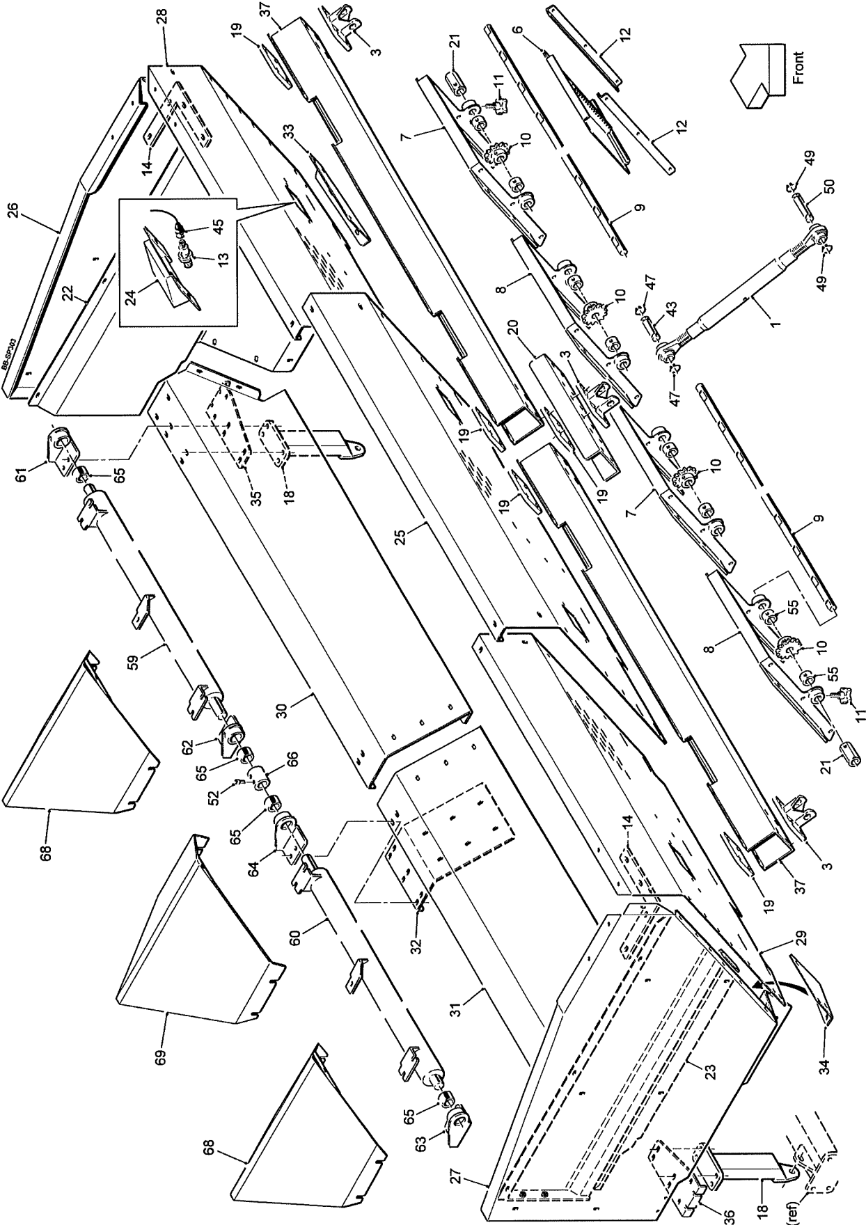
Hopper (front section) Assy No 65738
