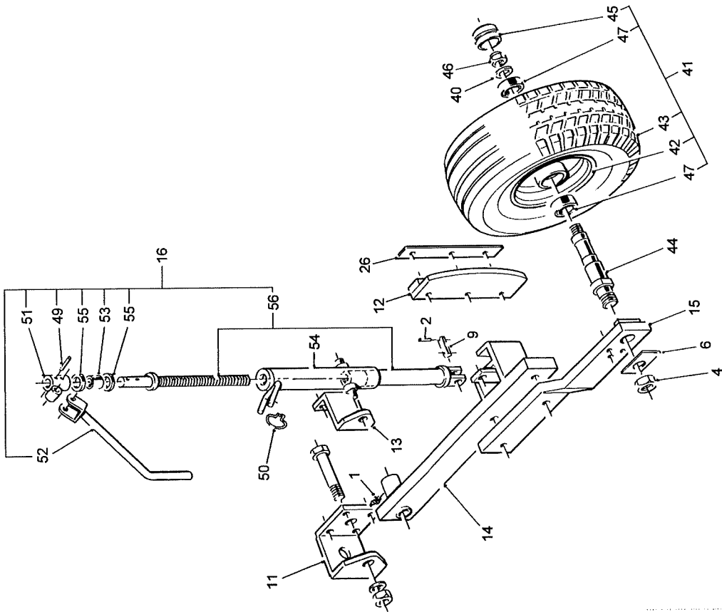
Outer wheel (drawn as LH unit)
