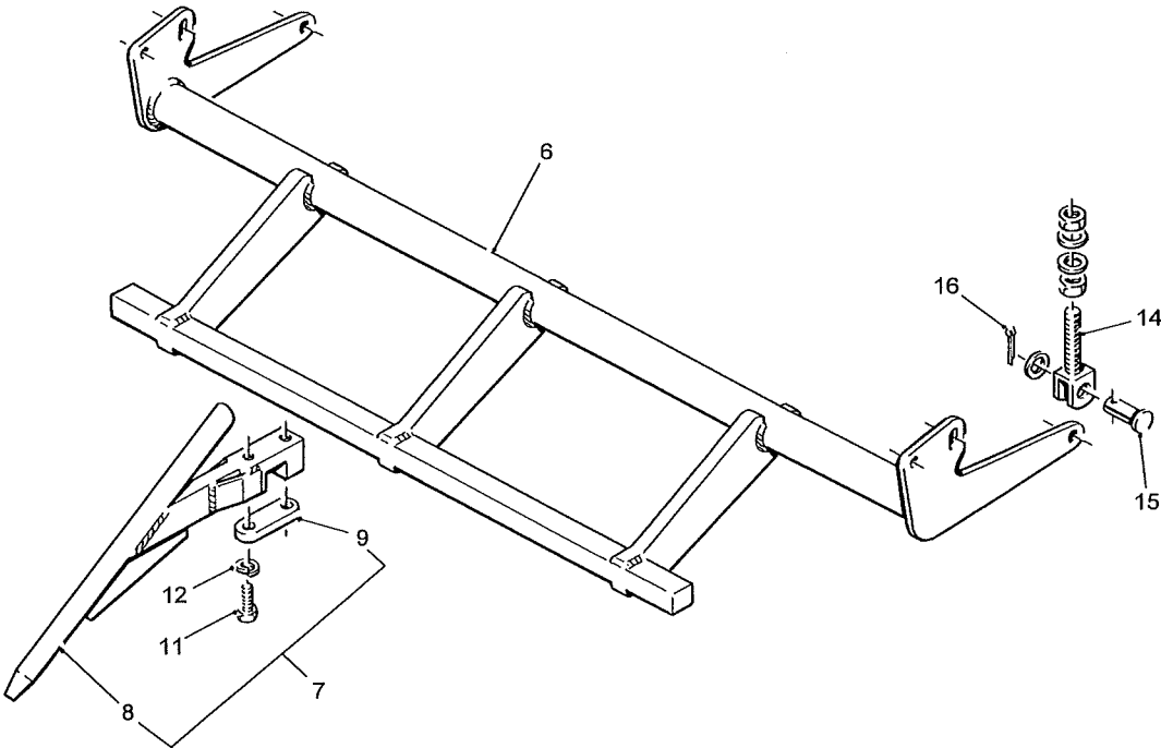
DETACHABLE CARROT PIN SHARE
